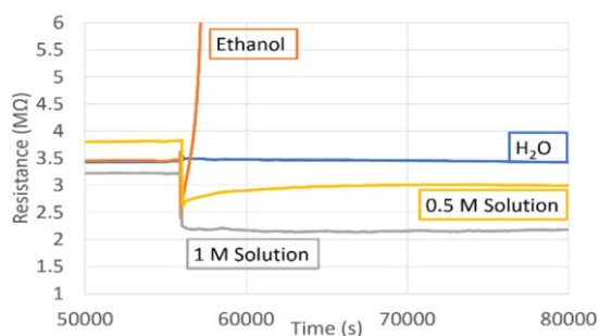
Figure 6: Behaviour of the sensors in presence of different analytes (water, ethanol, \text{NH}_4\text{OH} 1 M and 0.5 M).
